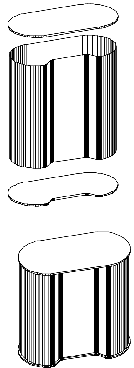
Double D workstation with one piece wrap and kneehole shaped base
